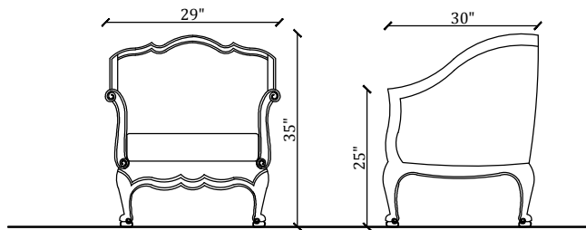
SINGLE SEATER SOFA FRONT VIEW
